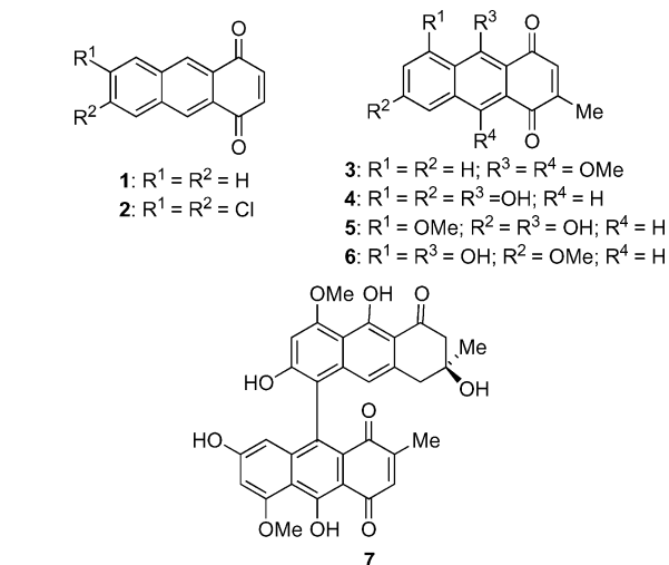
Figure 1. Structures of naturally occurring 1,4-anthraquinones.
