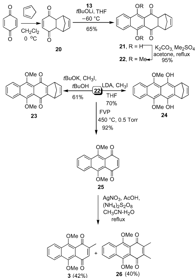
Scheme 4. Preparation of 9,10-dimethoxy-2-methyl-1,4-anthraquinone ( 3 ).
