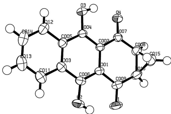
Figure 2. ORTEP diagram of compound 8 .
