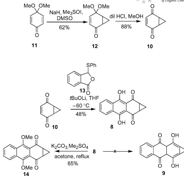
Scheme 1. Preparation of tetracyclic quinone 14 .
